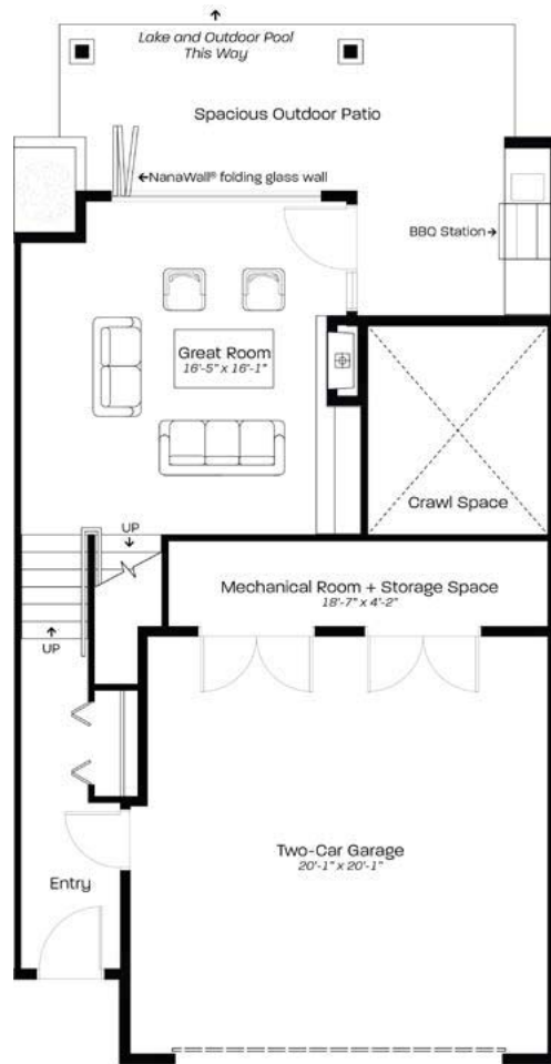
GROUND LEVEL
