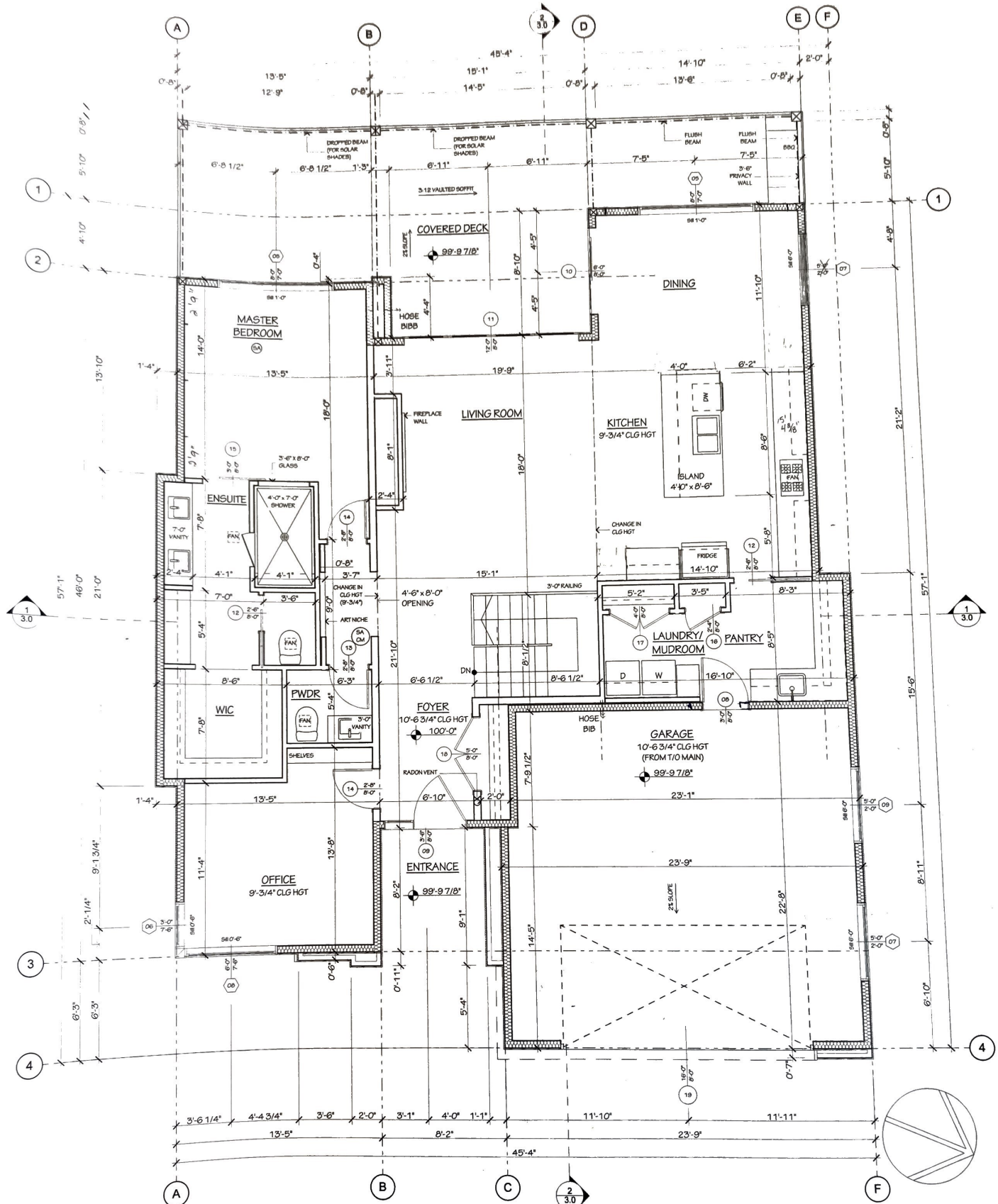
1 MAIN FLOOR PLAN SCALE: 1/4" = 1'-0"
